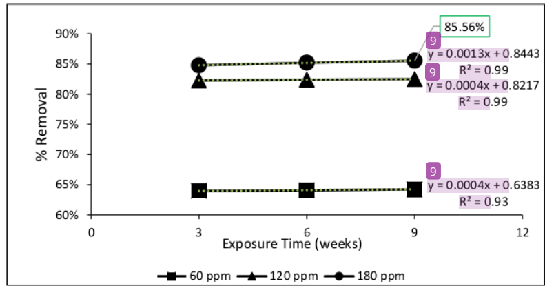
Figure 2. % Removal of Cu 2+ from soil.
