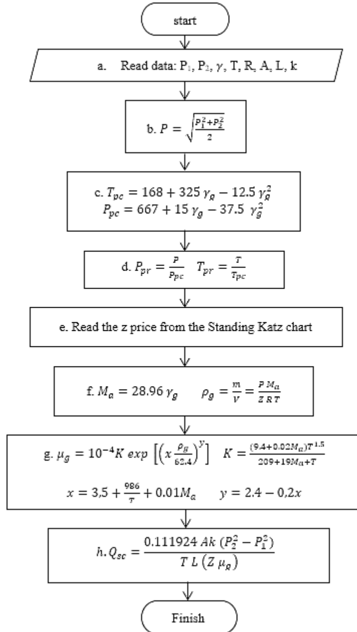
FIGURE 1. Flowchart of gas flow calculation in reservoir
