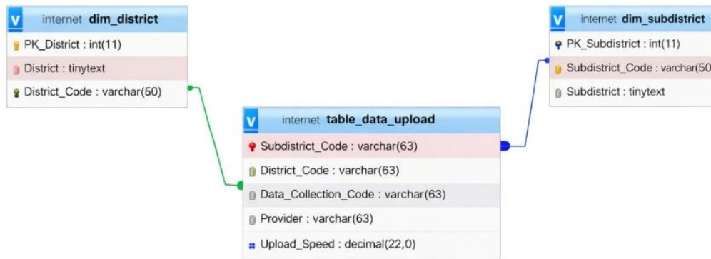
Figure 9. Star schema for upload speed data warehouse
