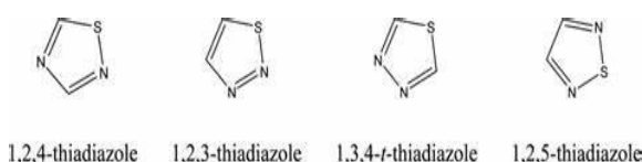
Figure (5): Thiadiazole isomers
