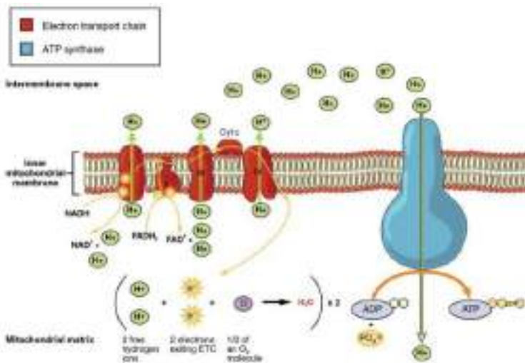
Gambar 7.7 Rantai transpor elektron (ETC) (Sumber: (Douglass College, 2021))
