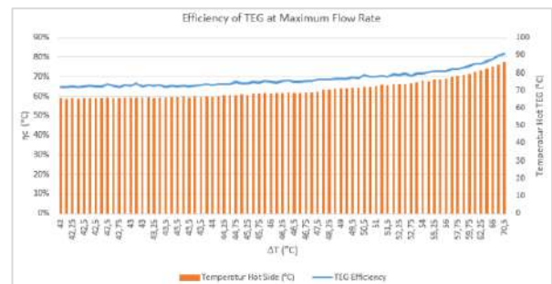
Figure 15. Efficiency of TEG at maximum flow rate.
