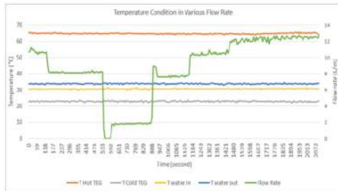
Figure 17. Temperature condition in various flow rate.
