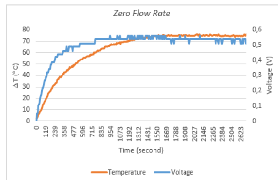
Figure 10. Voltage output TEG at zero flow rate.
