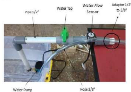
Figure 5. Structure cooler component
