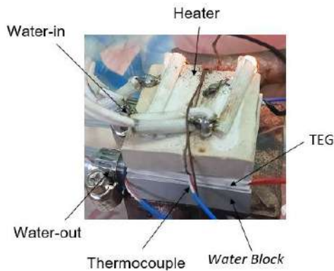
Figure 6. Water block position and the series
