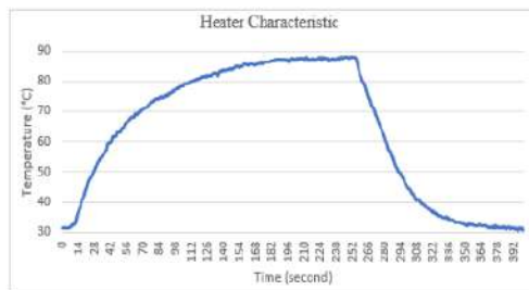
Figure 9. Heater characteristic.
