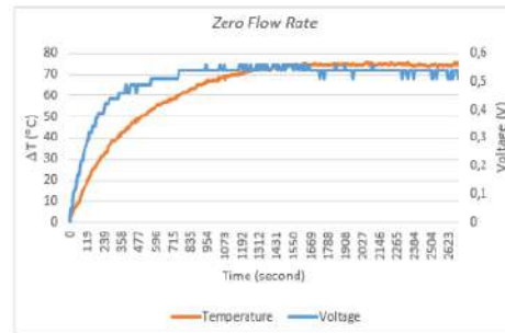
Figure 10. Voltage output TEG at zero flow rate.
