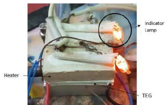
Figure 4. Heater system.
