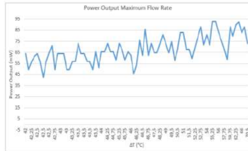
Figure 14. Power characteristics at maximum flow rate.
