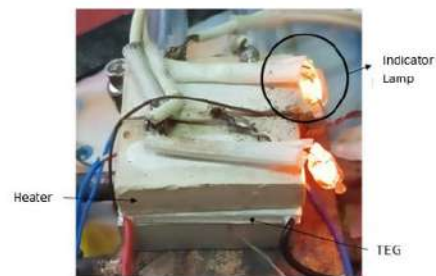
Figure 4. Heater system.
