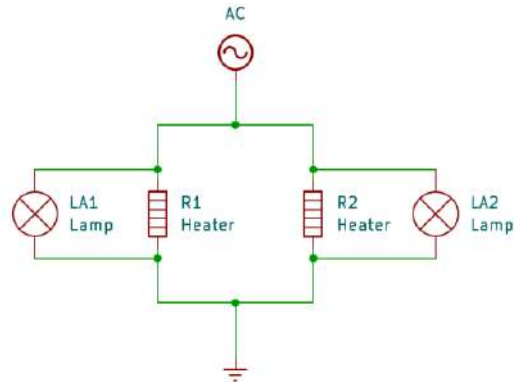
Figure 3. Wiring diagram heater.
