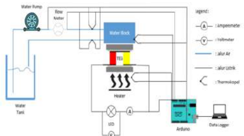
Figure 7. Design of TEG testing equipment.
