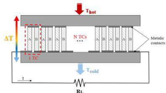
Figure 8. Temperature system TEG.
