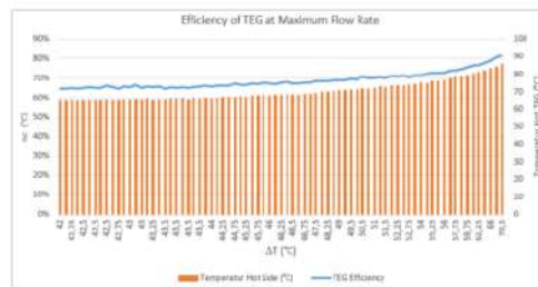
Figure 15. Efficiency of TEG at maximum flow rate.
