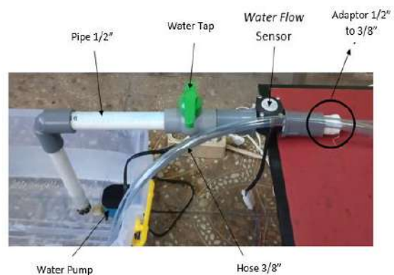
Figure 5. Structure cooler component
