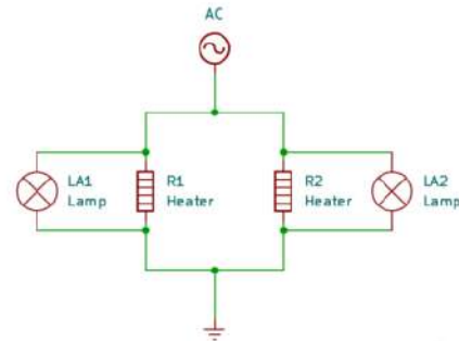
Figure 3. Wiring diagram heater.
