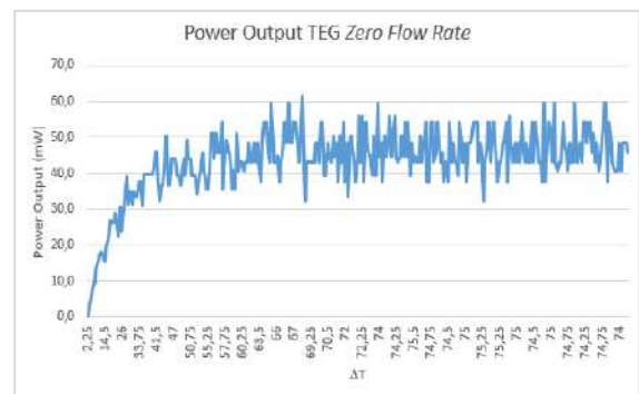
Figure 11. Power characteristics at zero flow rate.
