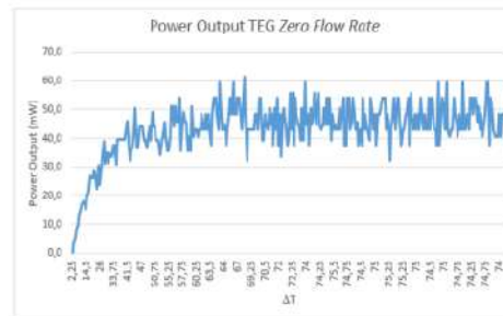
Figure 11. Power characteristics at zero flow rate.
