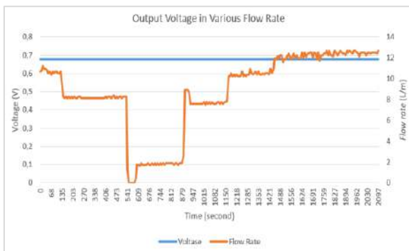
Figure 16. Output voltage in various flow rate.
