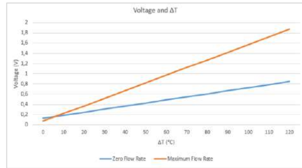
Figure 18. Output voltage TEG SP1848 27145 SA.
