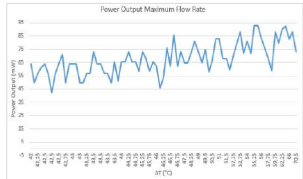
Figure 14. Power characteristics at maximum flow rate.
