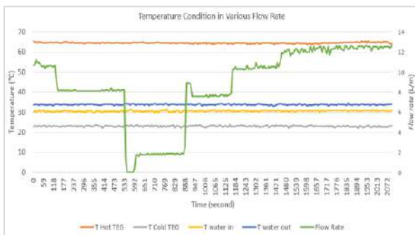
Figure 17. Temperature condition in various flow rate.
