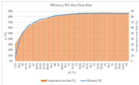
Figure 12. Efficiency of TEG at zero flow rate.
