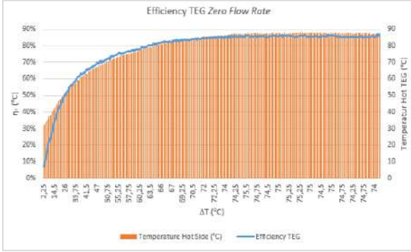
Figure 12. Efficiency of TEG at zero flow rate.
