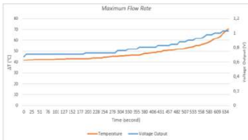
Figure 13. Voltage output at maximum flow rate.
