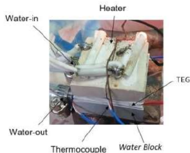
Figure 6. Water block position and the series
