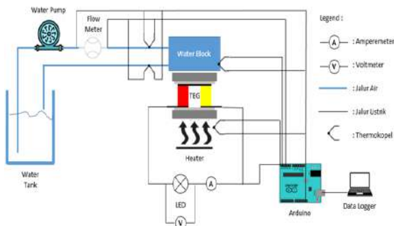
Figure 7. Design of TEG testing equipment.
