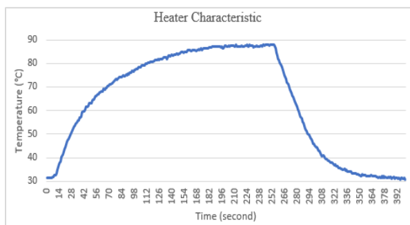
Figure 9. Heater characteristic.
