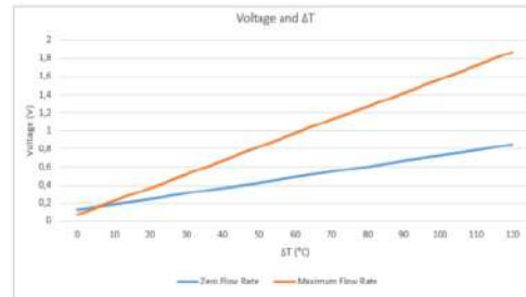
Figure 18. Output voltage TEG SP1848 27145 SA.
