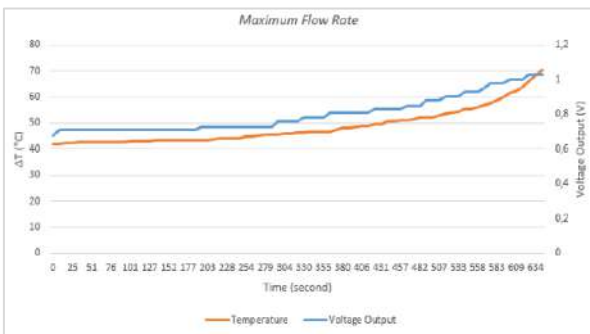
Figure 13. Voltage output at maximum flow rate.
