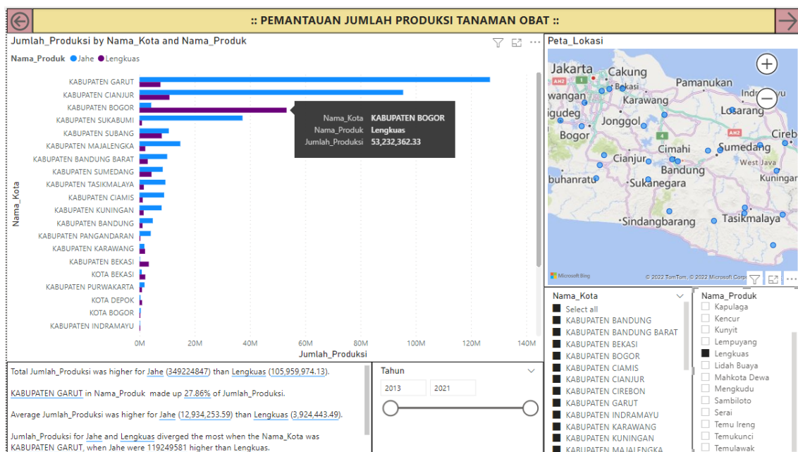
Gambar 14. Clustered Bar Chart Dashboard
