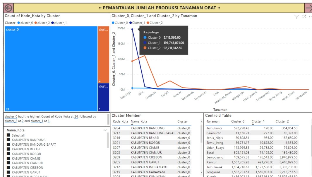
Gambar 18. Clustering Dashboard
