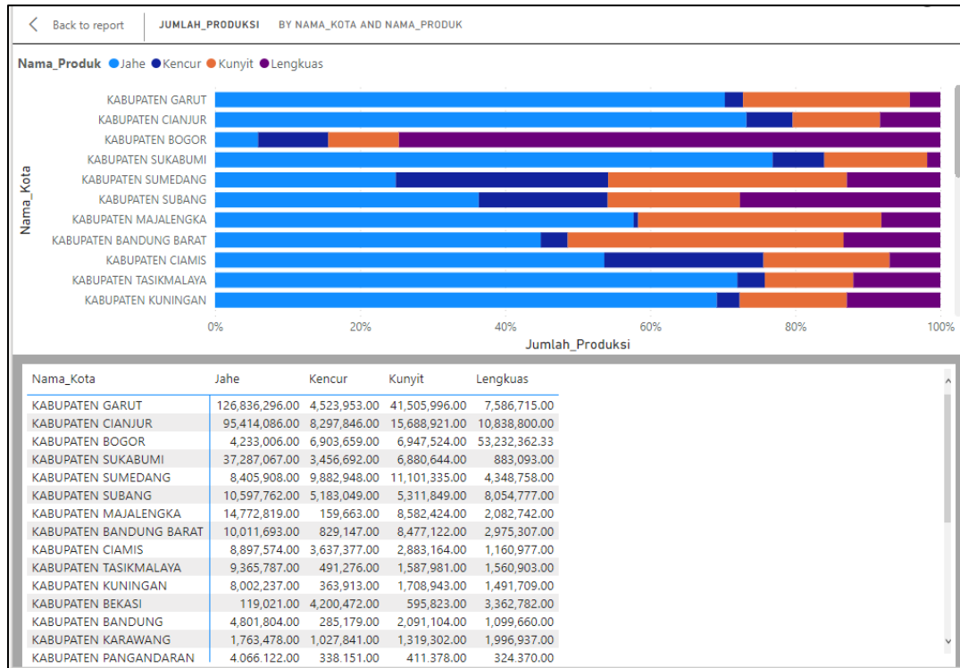
Gambar 17. Table Dashboard
