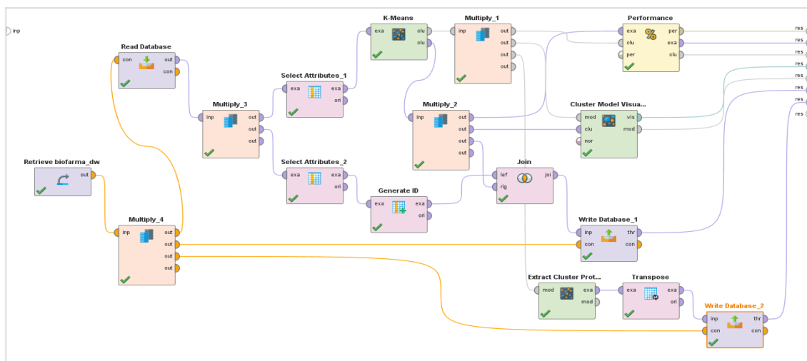
Gambar 10. Rancangan Data Mining
