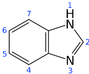
Fig. 1 benzimidazoles structure [6]
