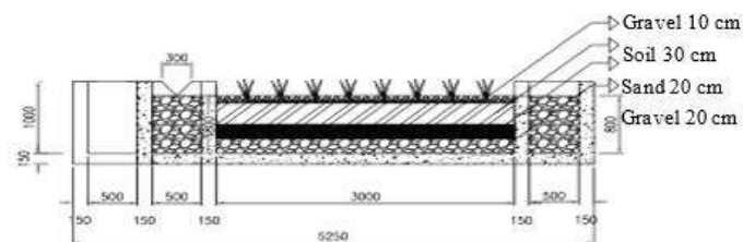
Figure 2. Constructed wetland reactor.
