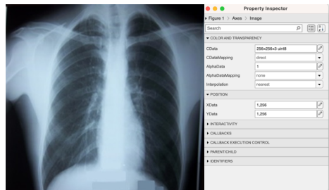
Figure 2. Resize Image
