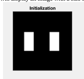
Figure 6. Initialization Mask
