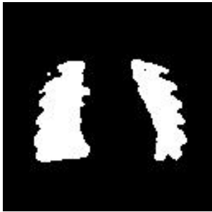
Figure 8. Chan-Vese Segmentation
