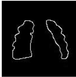
Figure 9. Canny Segmentation
