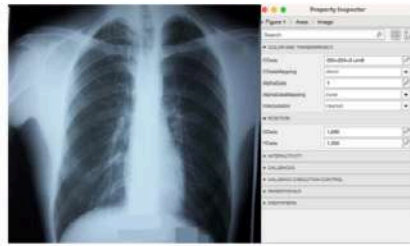
Figure 2. Resize Image
