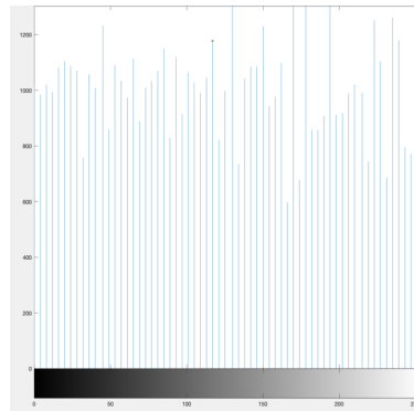
Figure 1. After Filtering
