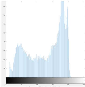
Figure 4. Before Filtering
