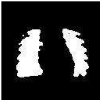
Figure 8. Chan-Vese Segmentation
