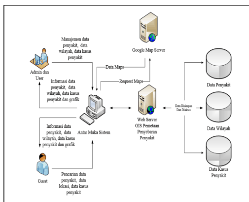
Fig 6. Overview of geographic information systems mapping the spread of disease
