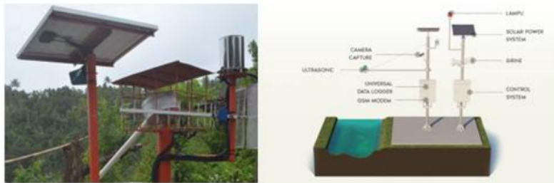
Gambar 13 Early Warning System Banjir
