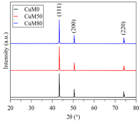
Figure 5. XRD results of CuM0, CuM50, and CuM80 samples
