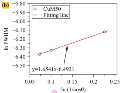
Figure 6. Calculation vs observation of diffraction pattern of the CuM50 sample (a) and Plot of \ln(1/\cos \theta) vs \ln FWHM of the CuM50 sample (b)
