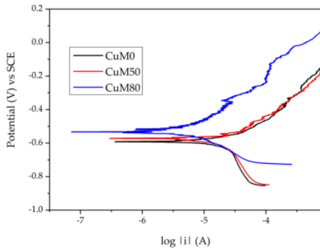
Figure 7. Polarization potentiodynamic test results
