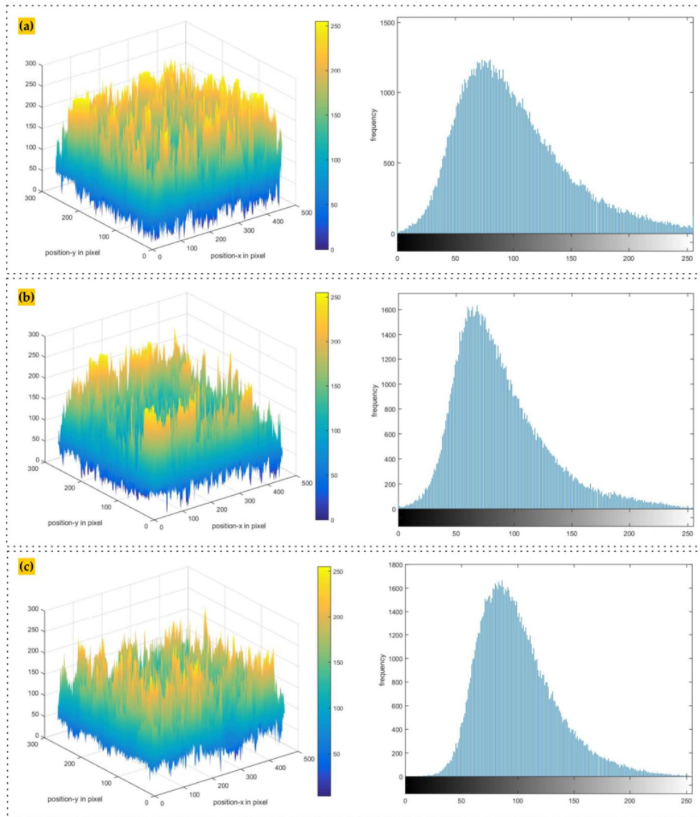
Figure 4. Roughness analysis results and histogram (a) CuM0, (b) CuM50, and (c) CuM80
