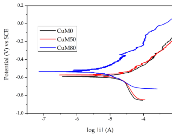
Figure 7. Polarization potentiodynamic test results
