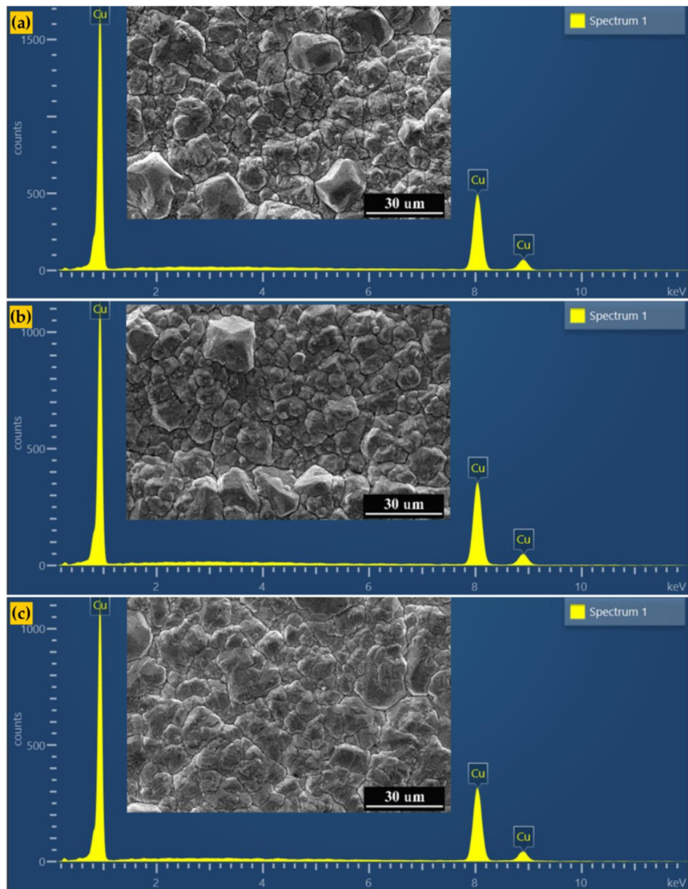
Figure 3. SEM-EDS results: (a) CuM0, (b) CuM50, and (c) CuM80
