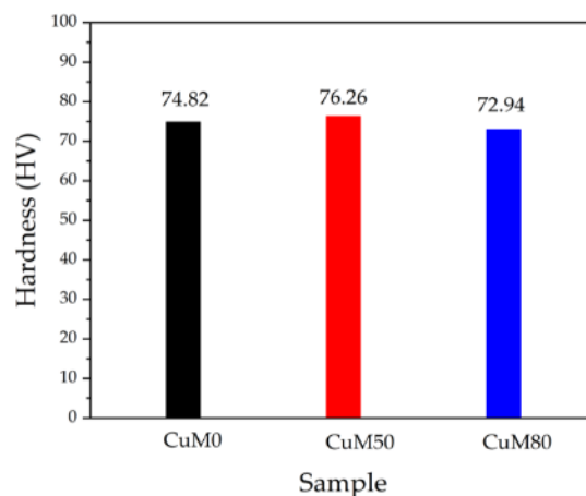
Figure 8. Hardness test results
