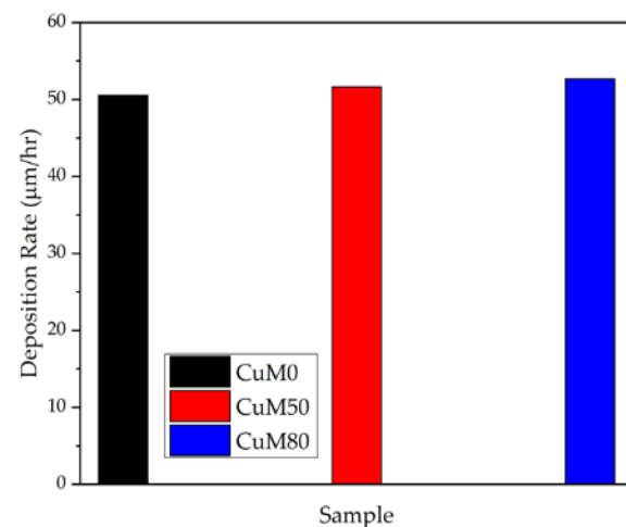
Figure 2. Deposition rates of the sample
