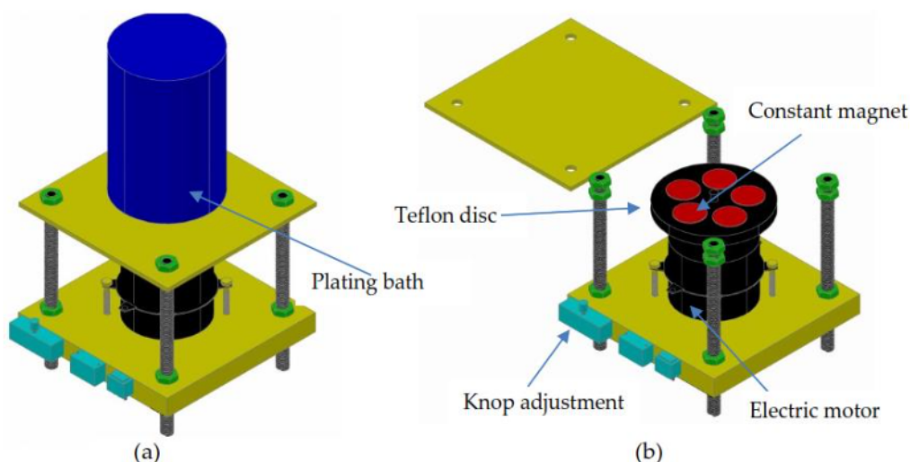
Figure 1. The apparatus of the electrodeposition process: (a) complete apparatus and (b) magnet position
