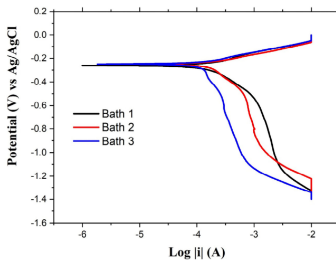
Figure 7. Corrosion curve for various samples
