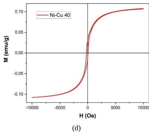
Figure 9. Hysteresis loops of multilayers generated at different current densities
