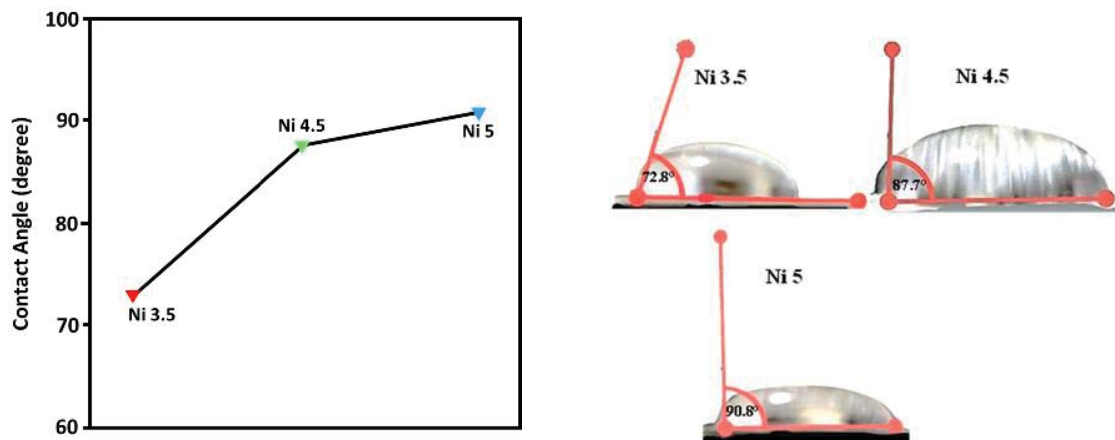
Figure 4: Wettability of the various Ni films deposited on the Al alloy substrates at different time.
