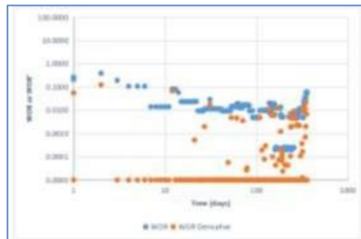
Figure 3. Diagnostic Plot ZNC Field
