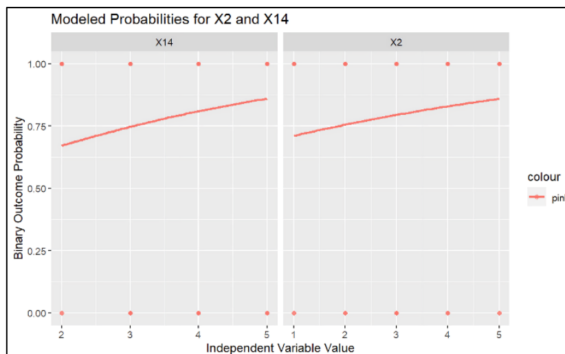
Figure 2. Prediction model
