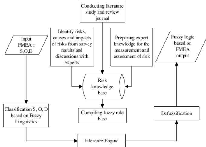
Figure 8. Architecture fuzzy linguistic model on risk assessment
