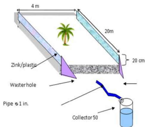
Fig. 1. Sediment collector; source: own elaboration
