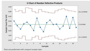
Figure 5. U control chart data plot
