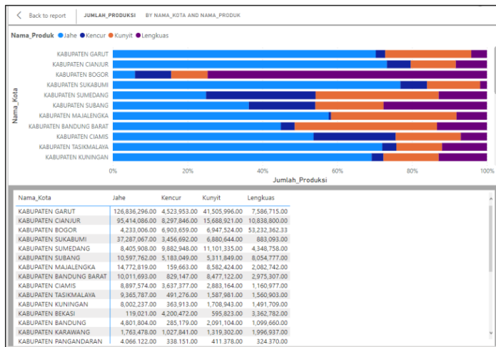
Gambar 17. Table Dashboard
