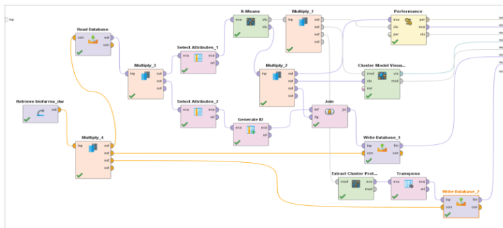
Gambar 10. Rancangan Data Mining
