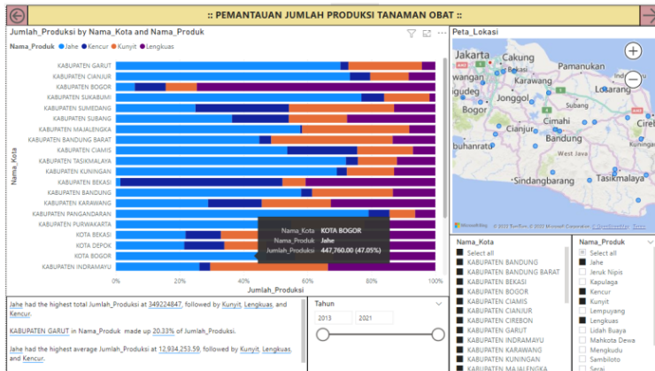
Gambar 12. Stacked Bar Chart Dashboard
