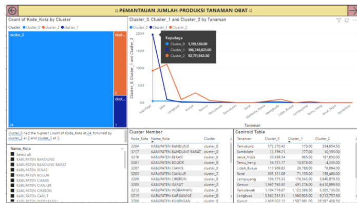
Gambar 18. Clustering Dashboard
