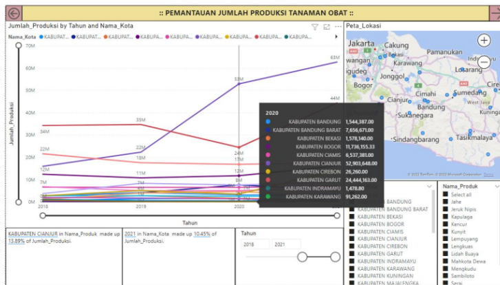
Gambar 16. Line Chart Dashboard
