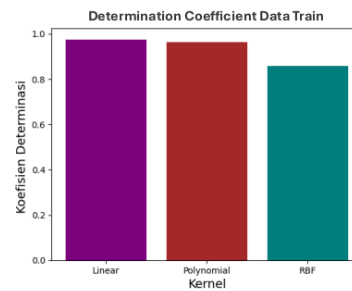
Figure 5. Comparison graph of Kernel data training function
