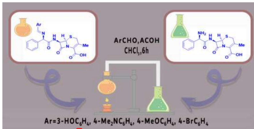
Scheme 2: Synthesis of cephalosporin Schiff bases 1–4.
