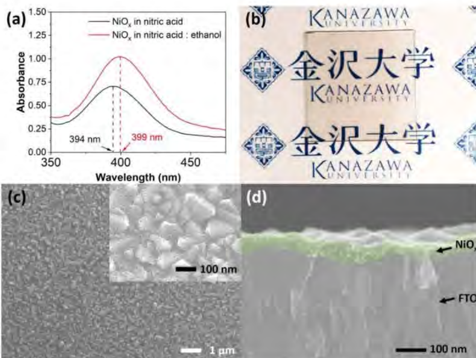
Fig. 2. (Color online) (a) The UV-vis spectra for NiO x in nitric acid and nitric acid with ethanol, (b) NiO x thin film appearance after annealing, (c) top view SEM image of NiO x thin film, and (d) cross-sectional SEM image of NiO x thin film on FTO.
