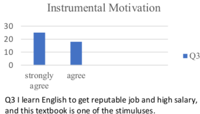
Fig. 4. Instrumental Motivation
