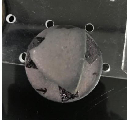
Fig. 4. 30% NSP Concrete sample for SEM.
