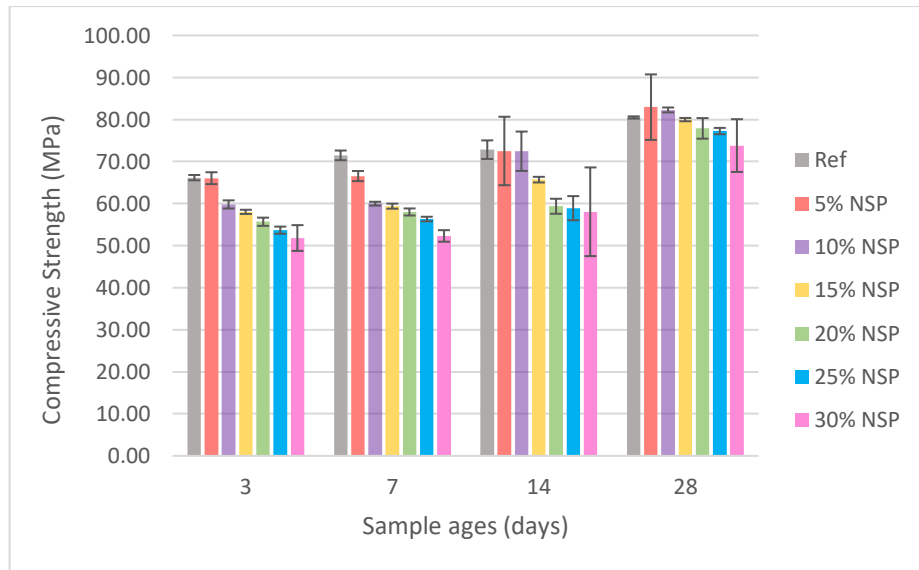
Fig. 5. Compressive Strength result.
