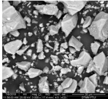
Fig. 6. Magnitude 3000 times of nickel slag powder (NSP)
