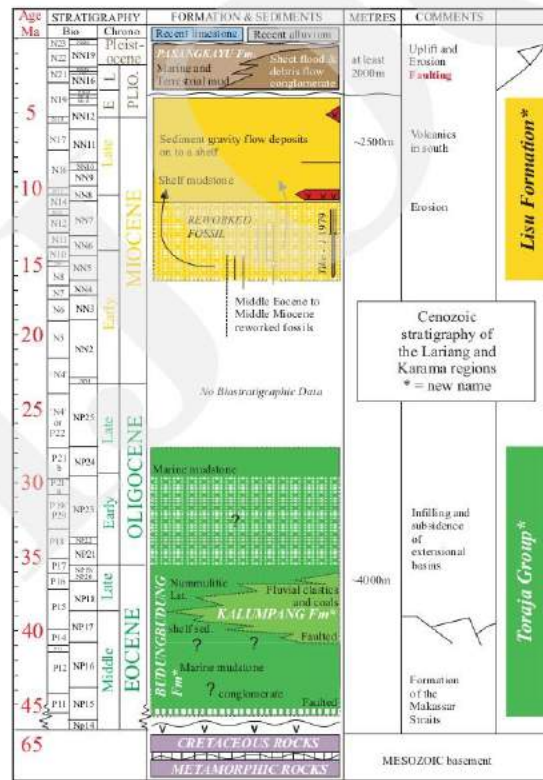
Figure 2. Stratigraphy of western Sulawesi (Calvert, 2000).
