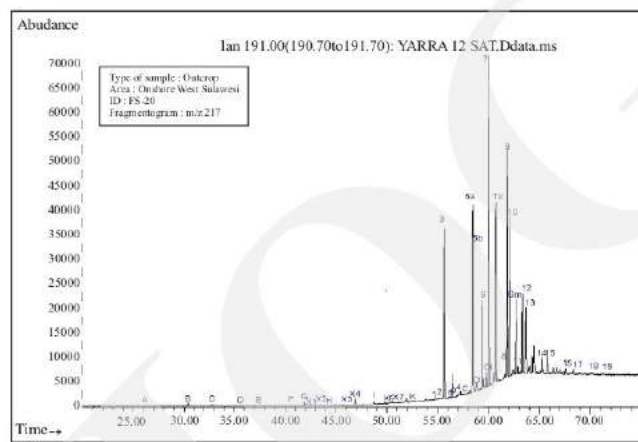
Figure 6. m/z 217 partial mass chromatograms showing sterane distribution of FS-20. See Table 2 for key to labels.
