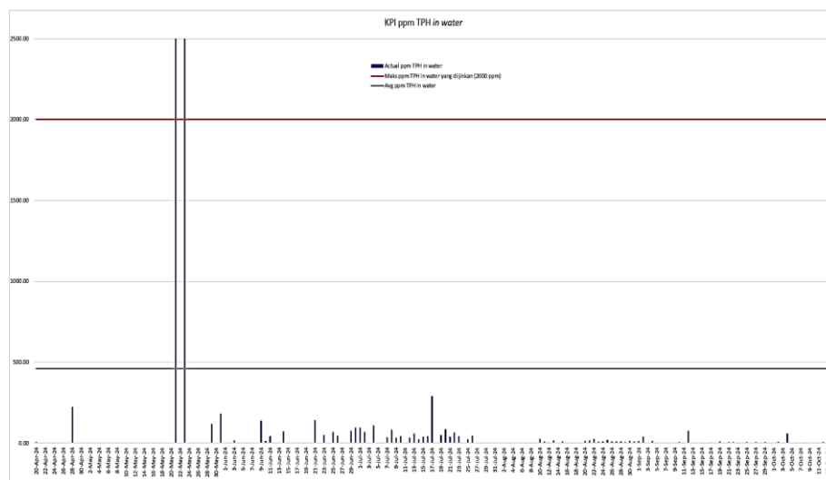
Figure 14. KPI ppm TPH in water
