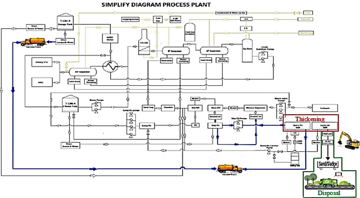
Figure 2. A simple diagram of the initial process of sludge management (Soetikno, A., 2023)
