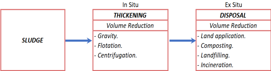
Figure 1. Initial sludge management method (Wiratomo, M., 2024)
