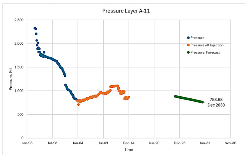
Figure 10. Pressure predicting of Well AX-02
