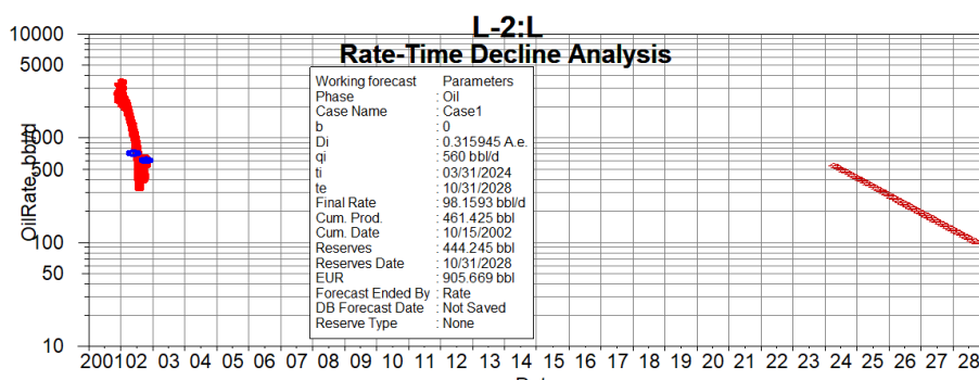
Figure 13. Decline Curve Analysis for Reservoir L-2
