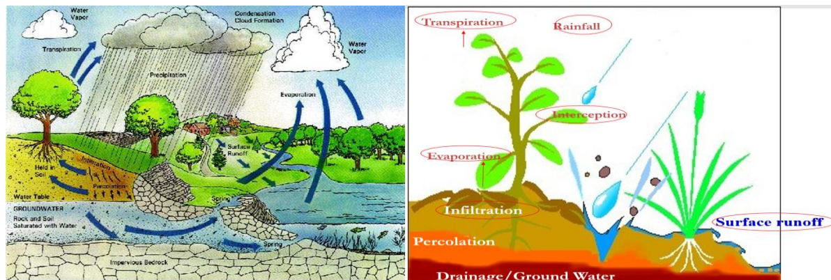
Figure 1. Hydrological Cycle
