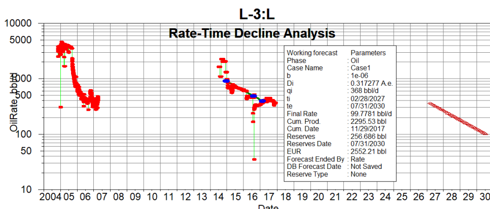
Figure 14. Decline Curve Analysis for Reservoir L-3
