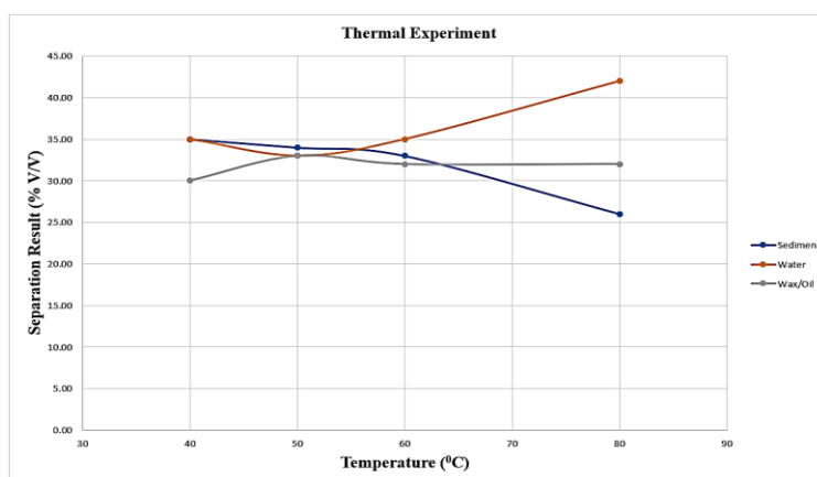
Figure 8. Stabilization through heat treatment
