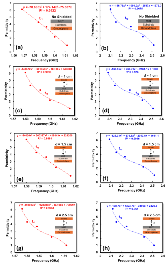
FIGURE 14. Polynomial equation based on resonant frequency and permittivity; (a) without shielded for f_{r1} , (b) without shielded for f_{r2} , (c) with cooper shielded of d = 1 cm for f_{r1} , (d) with cooper shielded of d = 1 cm for f_{r2} , (e) with cooper shielded of d = 1.5 cm for f_{r1} , (f) with cooper shielded of d = 1.5 cm for f_{r2} , (g) with cooper shielded of d = 2.5 cm for f_{r1} , (h) with cooper shielded of d = 2.5 cm for f_{r2}
