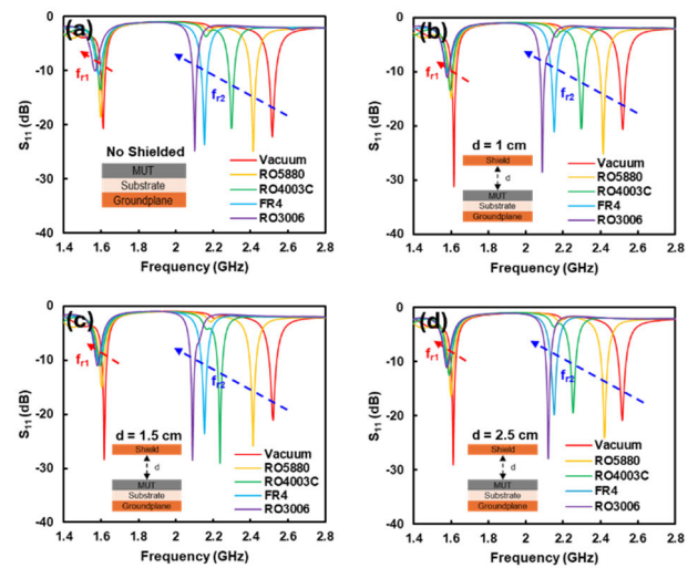
FIGURE 10. Shift of resonance frequency of proposed sensor; (a) without shielded, (b) with cooper shielded of d = 1 cm, (c) with cooper shielded of d = 1.5 cm, (d) with cooper shielded of d = 2.5 cm.
