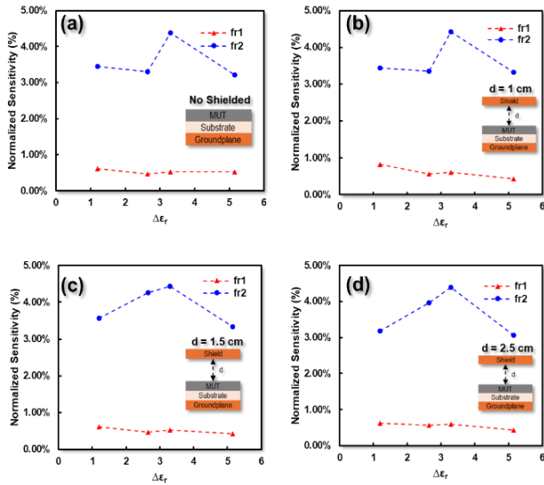
FIGURE 13. Normalized sensitivity of proposed sensor; (a) without shielded, (b) with cooper shielded of d = 1 cm, (c) with cooper shielded of d = 1.5 cm, (d) with cooper shielded of d = 2.5 cm
