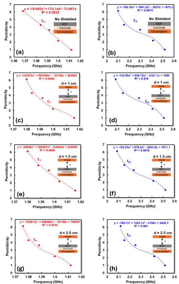
FIGURE 14. Polynomial equation based on resonant frequency and permittivity; (a) without shielded for f_{r1} , (b) without shielded for f_{r2} , (c) with copper shielded of d = 1\text{ cm} for f_{r1} , (d) with copper shielded of d = 1\text{ cm} for f_{r2} , (e) with copper shielded of d = 1.5\text{ cm} for f_{r1} , (f) with copper shielded of d = 1.5\text{ cm} for f_{r2} , (g) with copper shielded of d = 2.5\text{ cm} for f_{r1} , (h) with copper shielded of d = 2.5\text{ cm} for f_{r2} .
