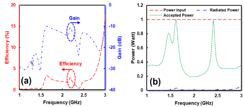
Fig. 3. Simulation result of single port resonator, (a) efficiency and gain of proposed resonator, (b) comparison between input, accepted dan transmitted power of proposed resonator
