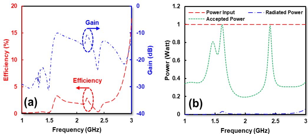
Fig. 1 Simulation result of single port resonator, (a) efficiency and gain of proposed resonator, (b) comparison between input, accepted dan transmitted power of proposed resonator
