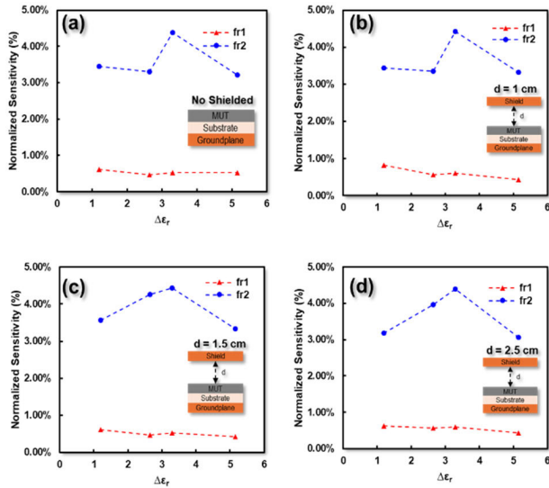
FIGURE 13. Normalized sensitivity of proposed sensor; (a) without shielded, (b) with copper shielded of d = 1\text{ cm} , (c) with copper shielded of d = 1.5\text{ cm} , (d) with copper shielded of d = 2.5\text{ cm} .
