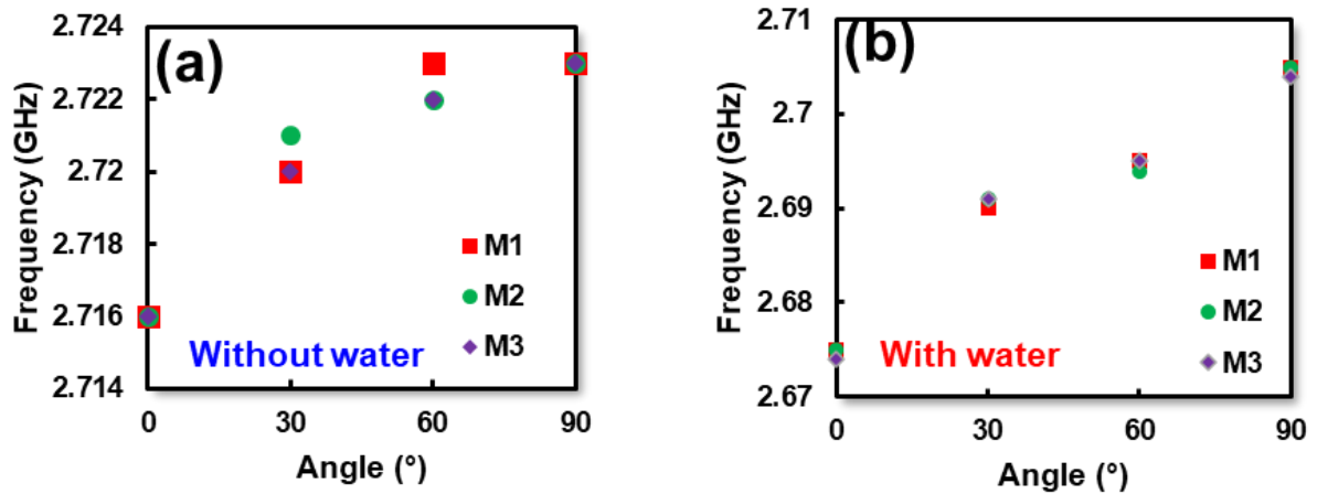
Fig.2 Repeatability measurement of bending detection; (a) without water, (b) with water
