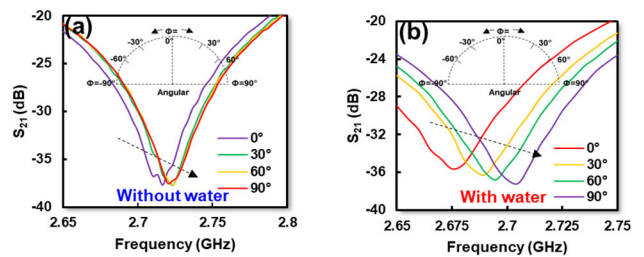
FIGURE 14. Measurement result of angular detection from 0^\circ - 90^\circ ; (a) without water, (b) with water.
