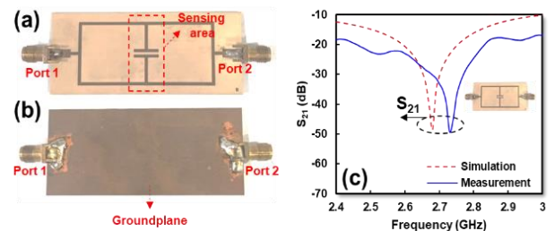
FIGURE 5. (a) Fabrication of ELC resonator at the front side, (b) fabrication of ELC resonator at the back side, (c) simulation and measurement of proposed resonator
