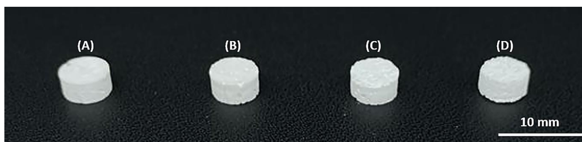
Figure 1. Composite blocks containing (A) 70% Sigma-Aldrich beta-tricalcium phosphate ( \beta -TCP) control with 30% polyacrylic acid (PAA) (SA-P), (B) 60% green mussel shell-derived \beta -TCP with 40% PAA (B60-P40), (C) 65% green mussel shell-derived \beta -TCP with 35% PAA (B65-P35), and (D) 70% green mussel shell-derived \beta -TCP with 30% PAA (B70-P30).
