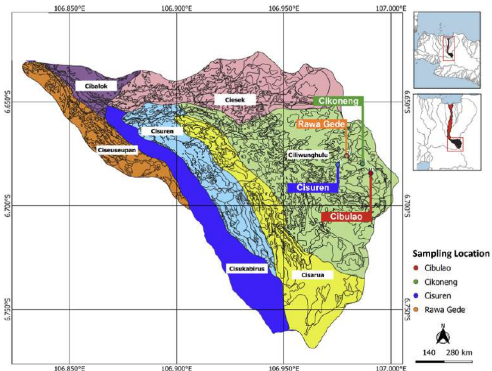
Figure 1. Study area (different colors showing different subwatersheds)
