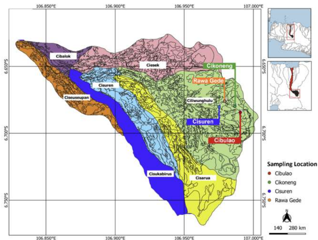
Figure 1. Study area (different colors showing different subwatersheds)
