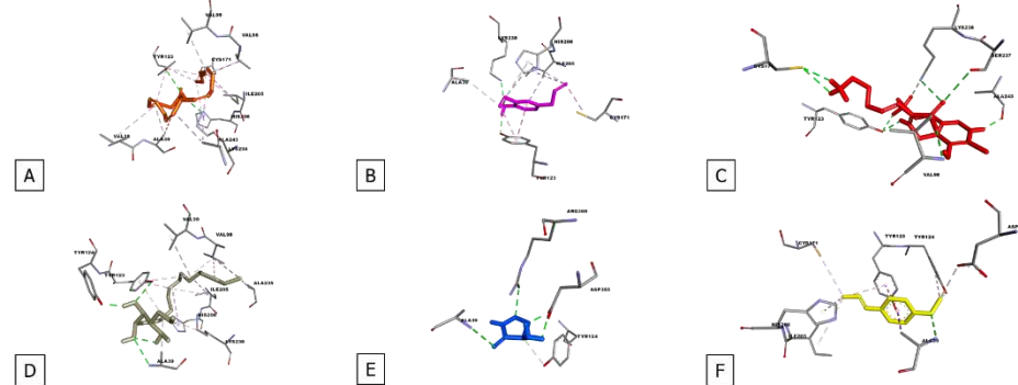
Figure 6. Molecular interactions of Cystalylin receptor with A. Arachidonic acid, B. eugenol, C. native ligand, D. phytosphingosine, E. positive control, and F. trans -anethole.
