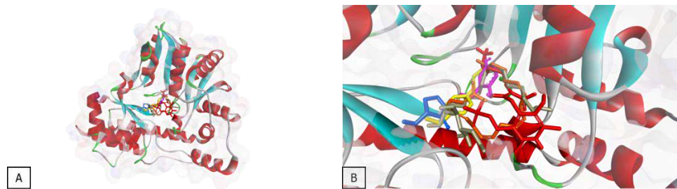
Figure 5. Conformations of the native ligand, M. oleifera compounds, and positive controls at Cystalylin A, ligand conformational positioning receptor, and B. Close-up view.
