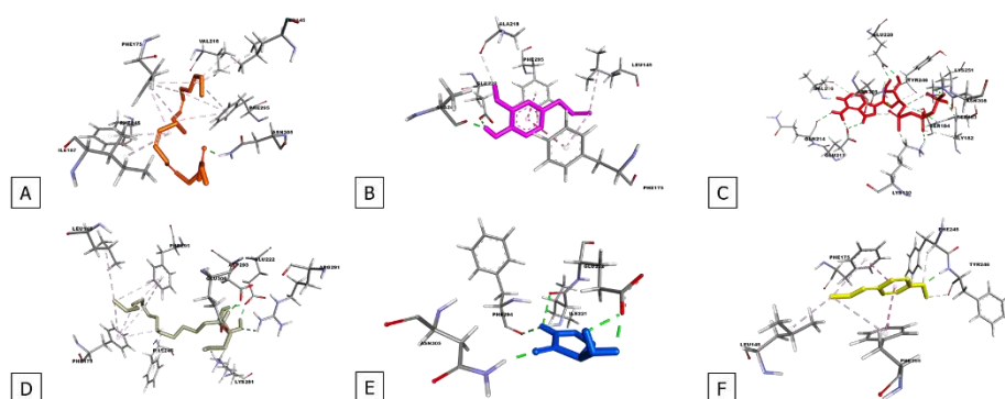
Figure 12. Molecular interactions of Ddl receptor with A. Arachidonic acid, B. eugenol, C. native ligand, D. phytosphingosine, E. positive control, and F. trans -anethole.
