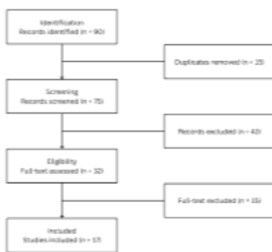
Gambar 1. Diagram PRISMA
