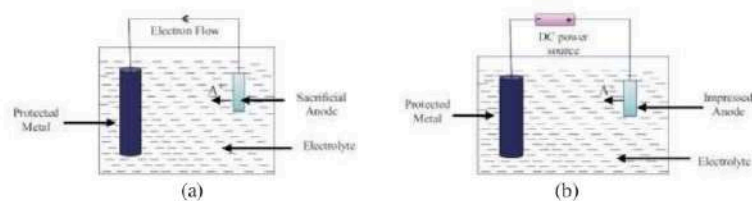
Figure 1. Sacrificial anode cathodic protection method: (a). Impressed anode cathodic (b) protection method [5]
