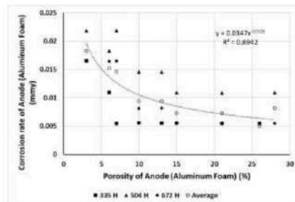
Figure 6. Corrosion rate anode versus porosity of anode (aluminum foam)
