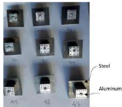
Figure 3. Galvanic Couple of cathode (steel)/anode (aluminum foam)
