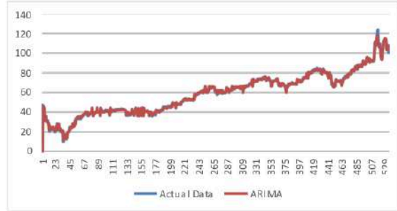
FIGURE 10. Plot Using ARIMA Method
