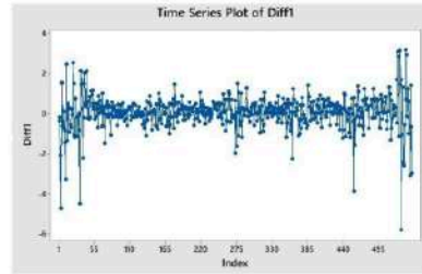
FIGURE 6. The Result of Differencing-Natural Logarithm Plot
