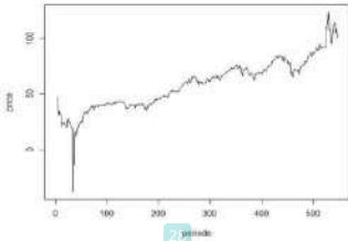
FIGURE 3. Time Series Plot
