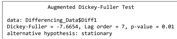
FIGURE 7. The Result of Differencing-Natural Logarithm by Using ADF Test
