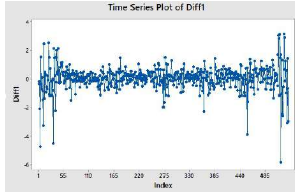
FIGURE 6. The Result of Differencing-Natural Logarithm Plot
