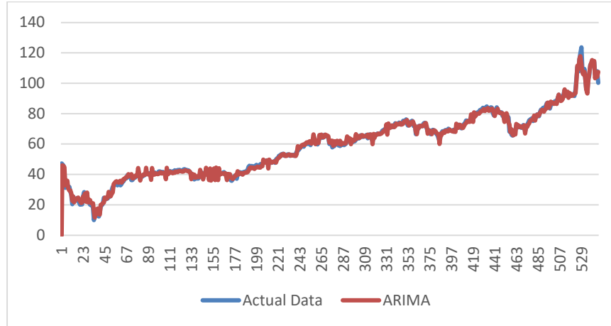
FIGURE 10. Plot Using ARIMA Method
