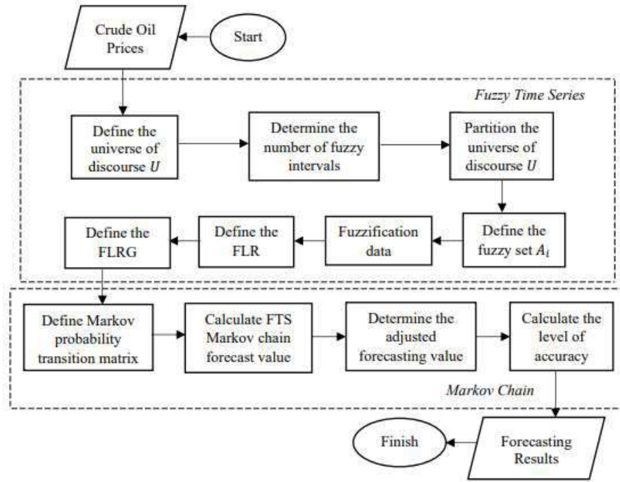
FIGURE 2. Flowchart of Fuzzy Time Series Markov Chain
