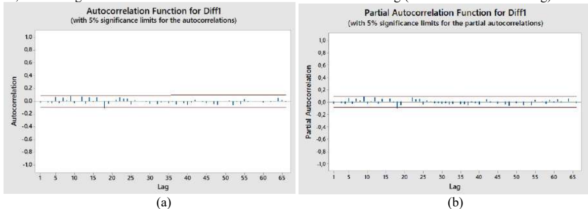
FIGURE 8. (a) ACF Plot & (b) PACF Plot After Natural Logarithm Differencing Process
