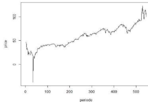
FIGURE 3. Time Series Plot
