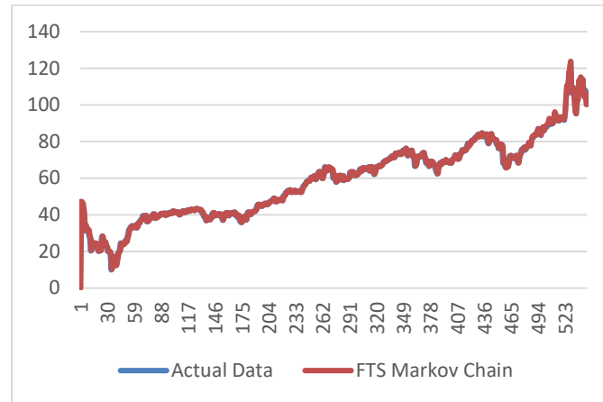
FIGURE 4. Plot Using FTS Markov Chain
