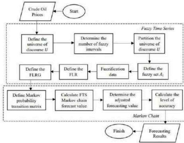
FIGURE 2. Flowchart of Fuzzy Time Series Markov Chain
