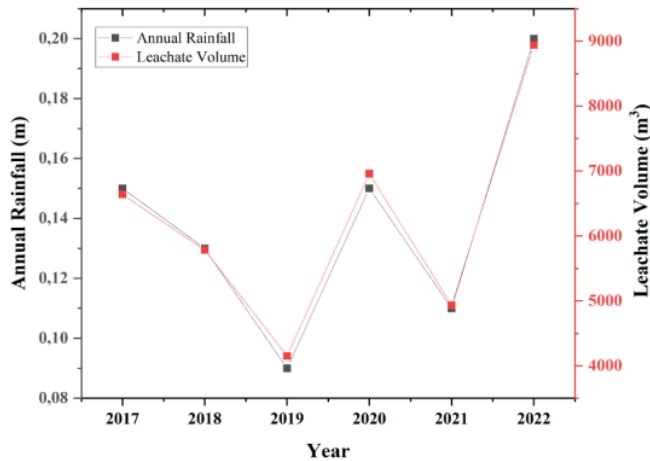
Figure 11. Relationship between leachate volume and annual rainfall
