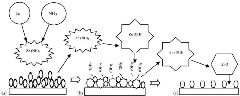
Figure 4. Mechanism of ZnO thin film growth [21].
