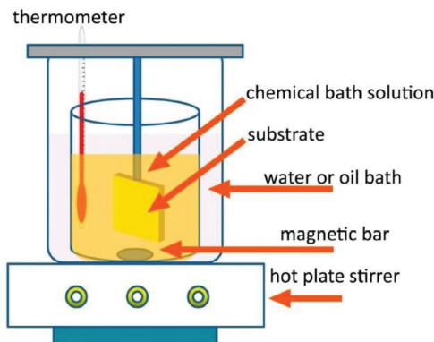
Figure 3. The arrangement of CBD equipment [16].
