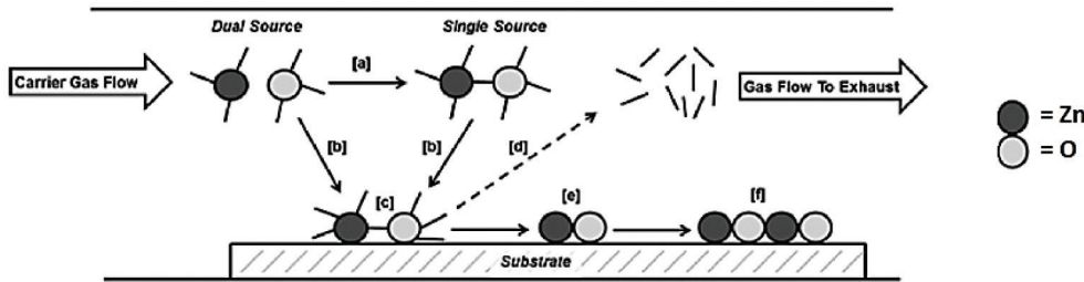
Figure 6. ZnO thin film fabrication. Mechanism with CVD [32].
