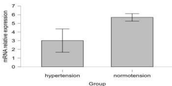
Figure 1. mRNA relative expression Sirtuin-I ( p < 0.05 )*
