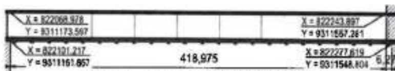
Picture 2. Layout of Quay Wall Structure
