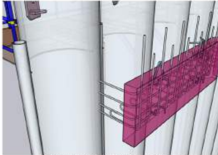
Picture 9. Clash Detection Coping Concrete
