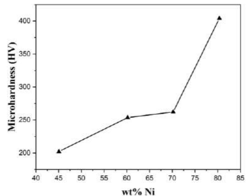
Figure 10. Relation wt% Ni vs microhardness
