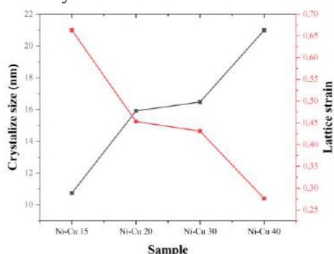
Figure 4. Ni-Cu lattice strain and size on Al at various current densities in the plating bath.
