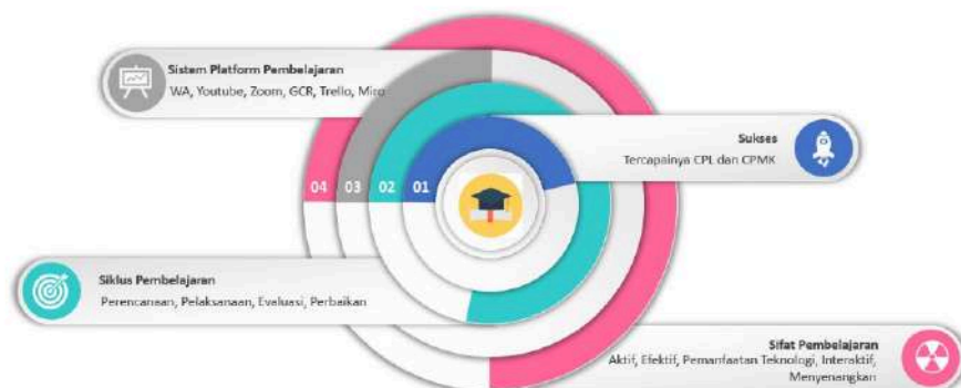
Gambar 1. ThreeS Framework
